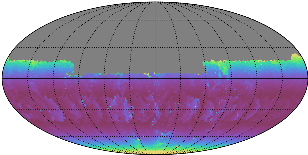
weather_cloudso18v3.4_10yrs Yr 1 u band: Min airmass
