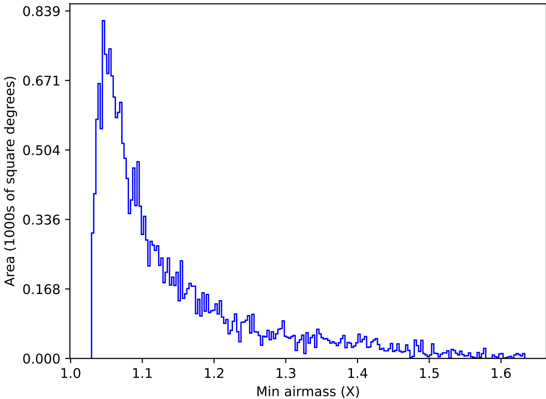
weather_cloudso18v3.4_10yrs Yr 1 u band: Min airmass
