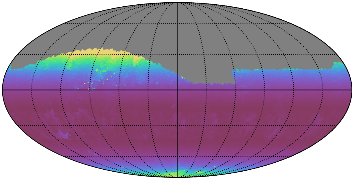
weather_cloudso18v3.4_10yrs Yr 1 r band: Min airmass
