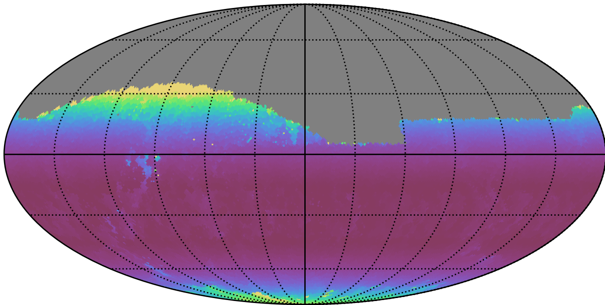
weather_cloudso18v3.4_10yrs Yr 1 i band: Min airmass
