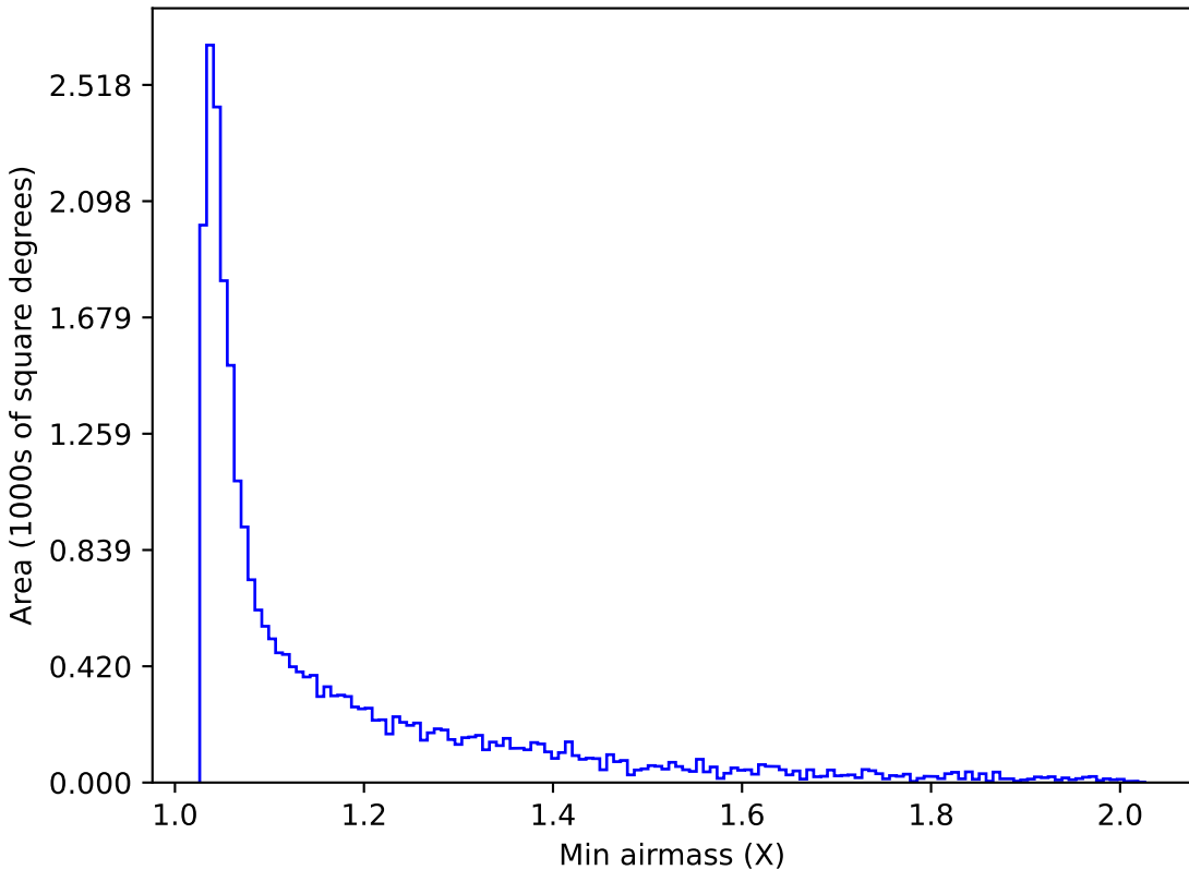
weather_cloudso18v3.4_10yrs Yr 1 i band: Min airmass
