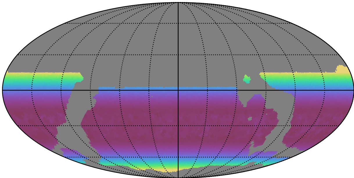
weather_cloudso18v3.4_10yrs WFD z band: Min airmass
