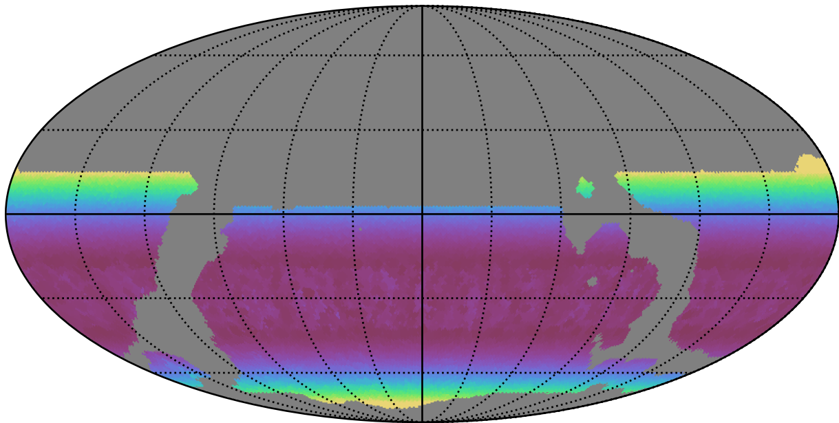
weather_cloudso18v3.4_10yrs WFD u band: Min airmass
