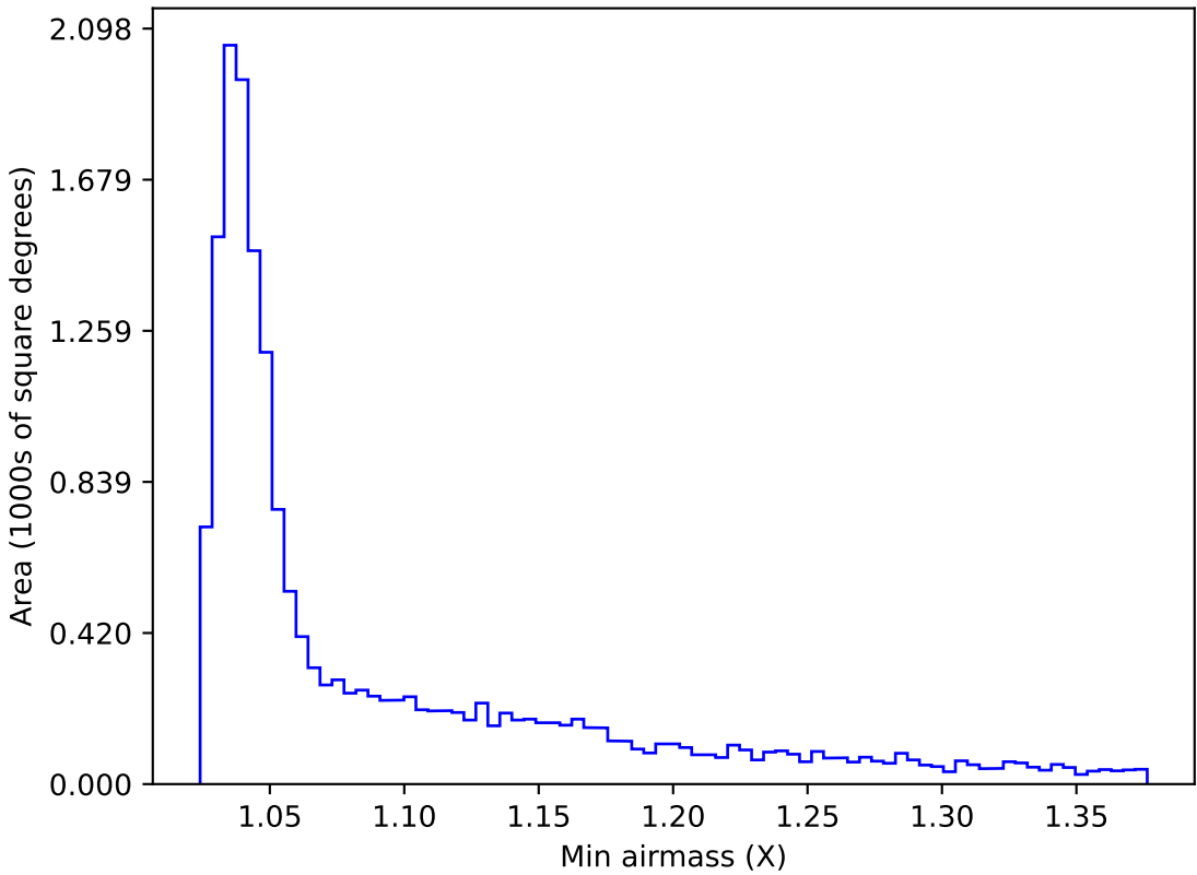
weather_cloudso18v3.4_10yrs WFD u band: Min airmass
