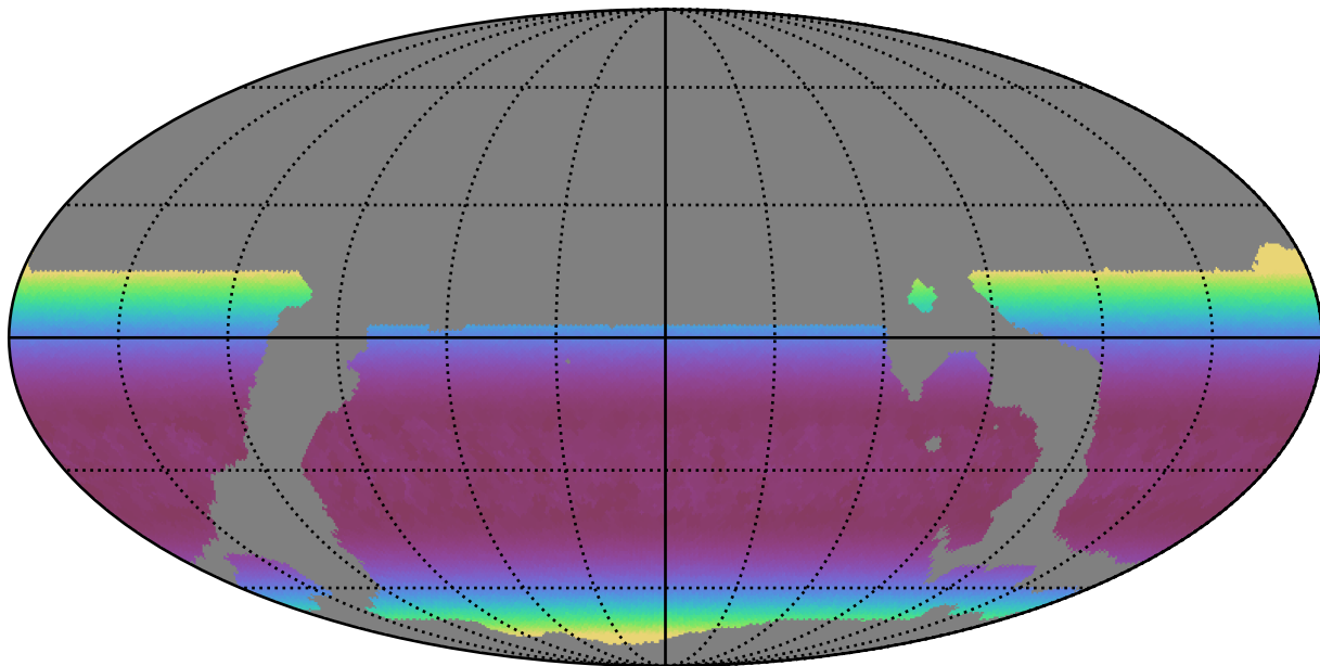
weather_cloudso18v3.4_10yrs WFD r band: Min airmass
