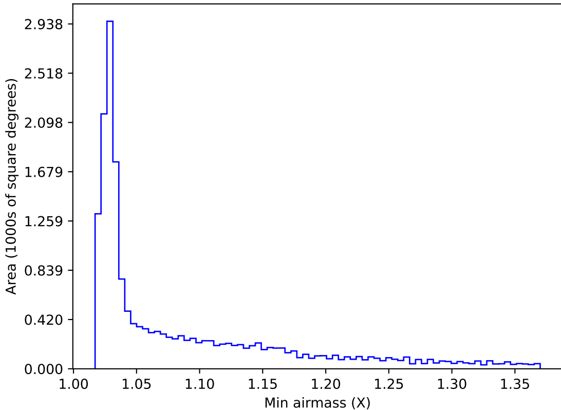
weather_cloudso18v3.4_10yrs WFD r band: Min airmass
