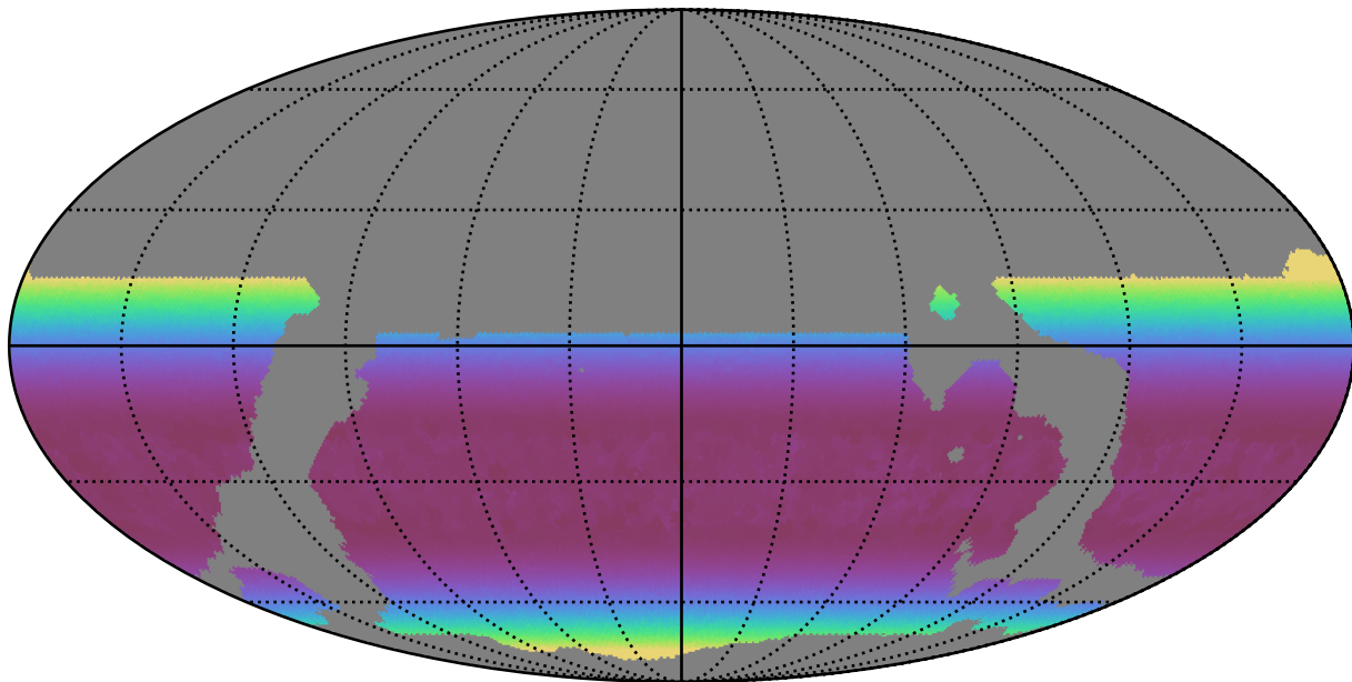
weather_cloudso18v3.4_10yrs WFD i band: Min airmass
