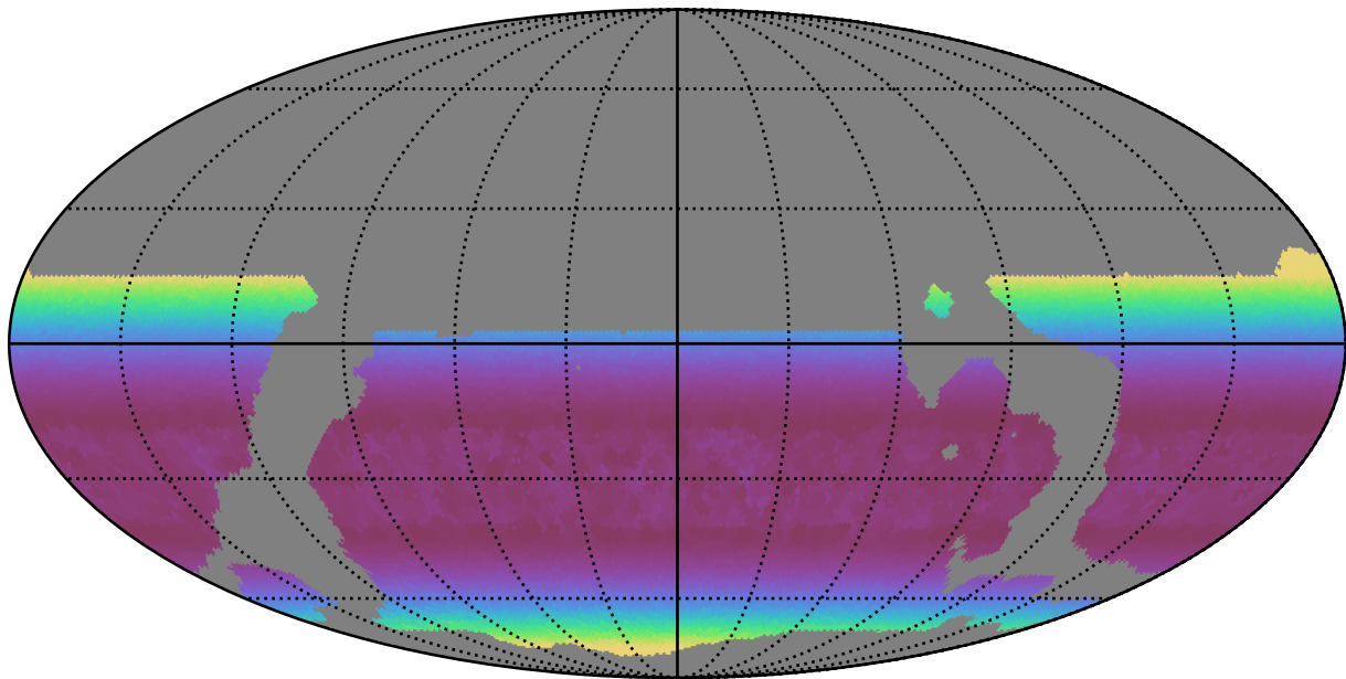
weather_cloudso18v3.4_10yrs WFD g band: Min airmass
