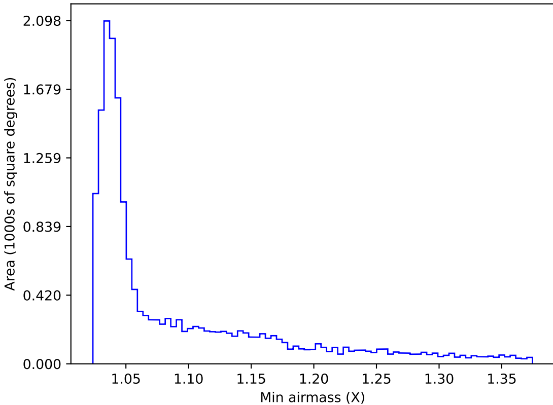
weather_cloudso18v3.4_10yrs WFD g band: Min airmass
