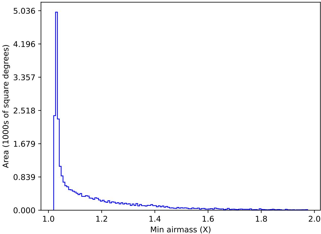
weather_cloudso18v3.4_10yrs All sky z band: Min airmass
