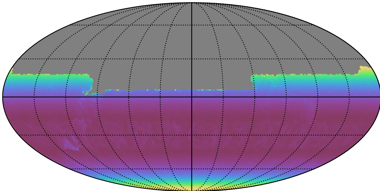
weather_cloudso18v3.4_10yrs All sky u band: Min airmass
