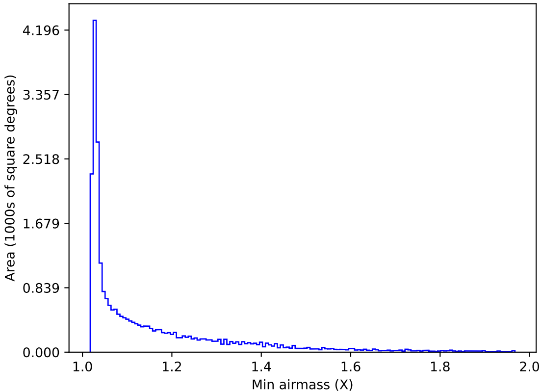
weather_cloudso18v3.4_10yrs All sky r band: Min airmass
