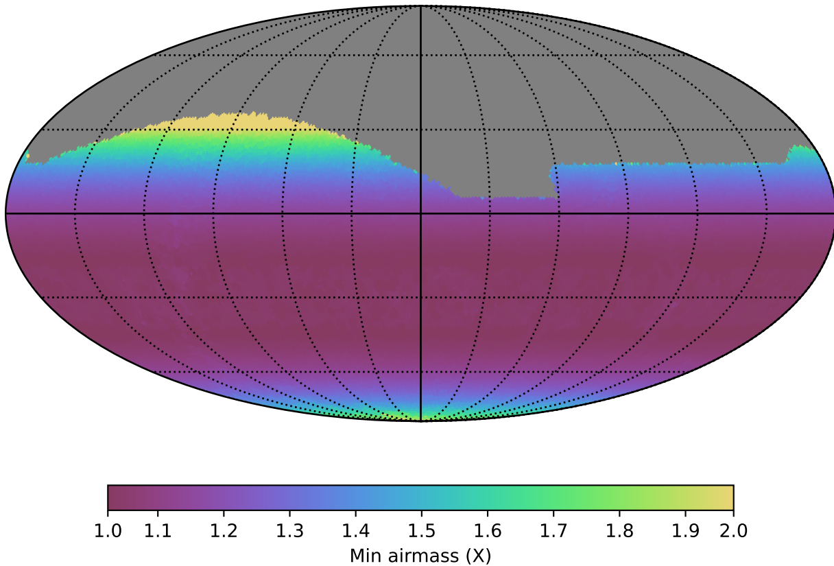
weather_cloudso18v3.4_10yrs All sky g band: Min airmass
