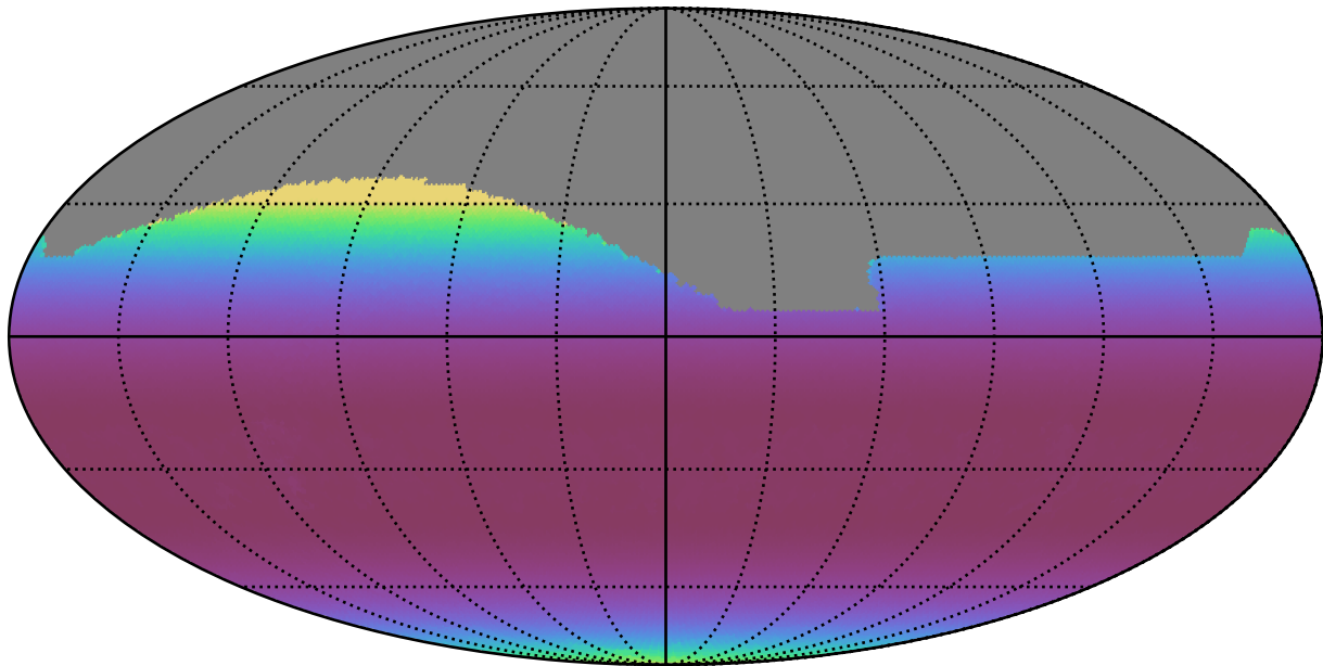
weather_cloudso18v3.4_10yrs All sky all bands: Min airmass
