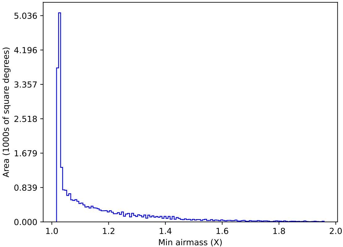
weather_cloudso18v3.4_10yrs All sky all bands: Min airmass
