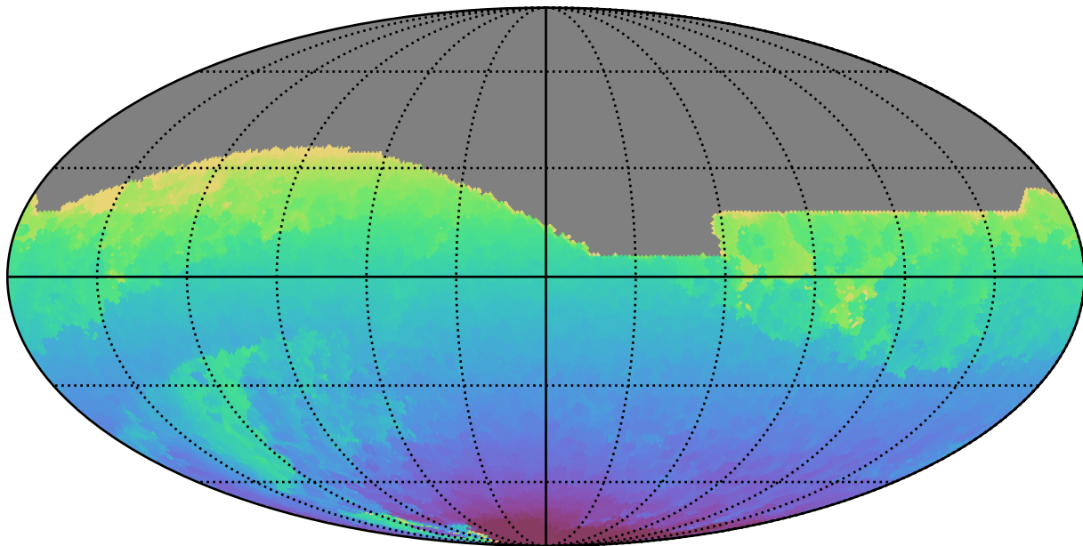
weather_cloudso18v3.4_10yrs All sky all bands: Min HA
