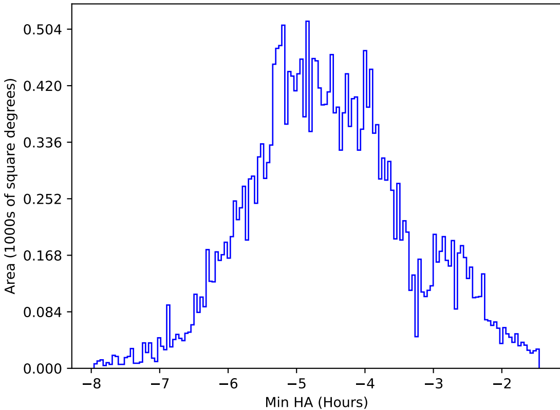
weather_cloudso18v3.4_10yrs All sky all bands: Min HA
