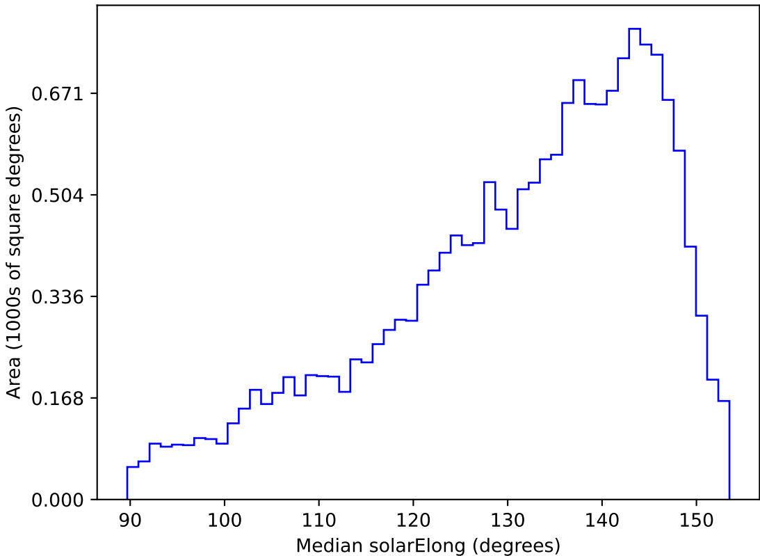
weather_cloudso18v3.4_10yrs WFD u band: Median solarElong
