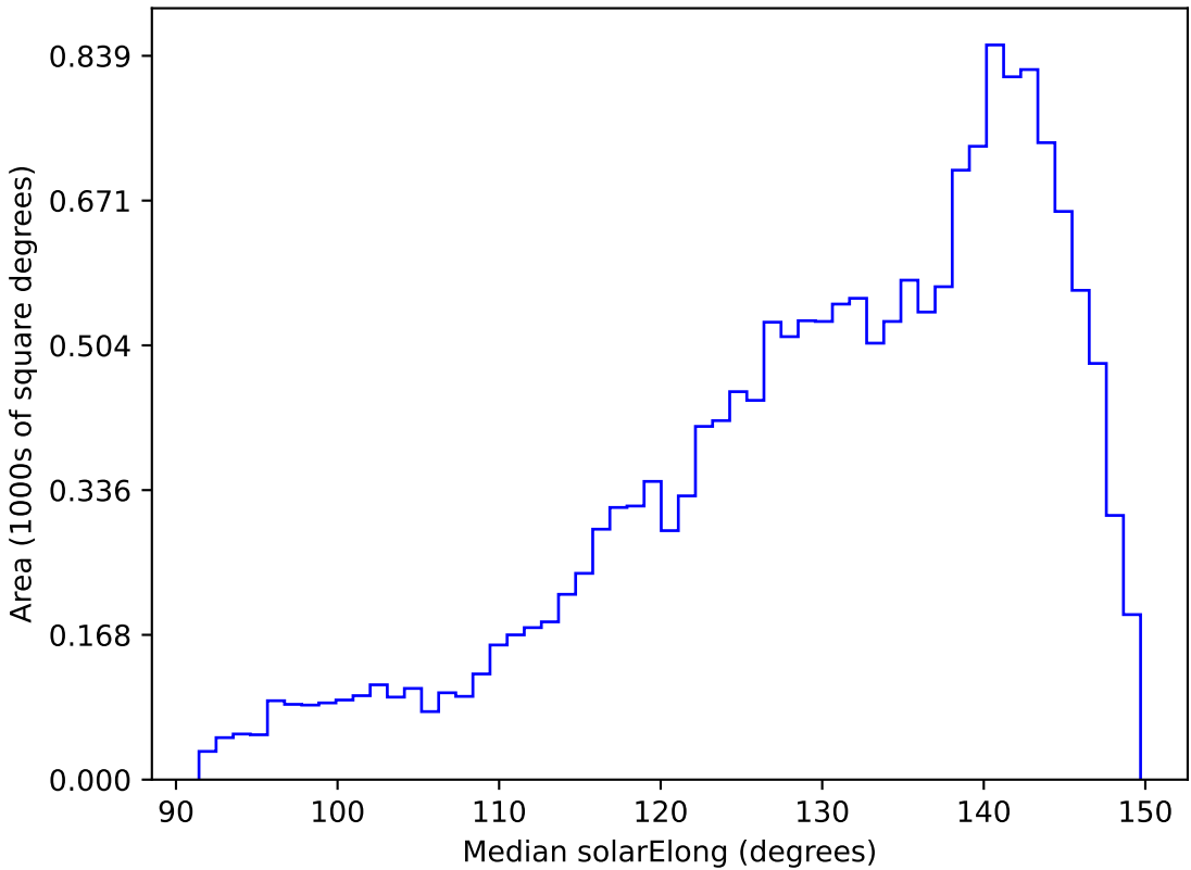
weather_cloudso18v3.4_10yrs WFD r band: Median solarElong
