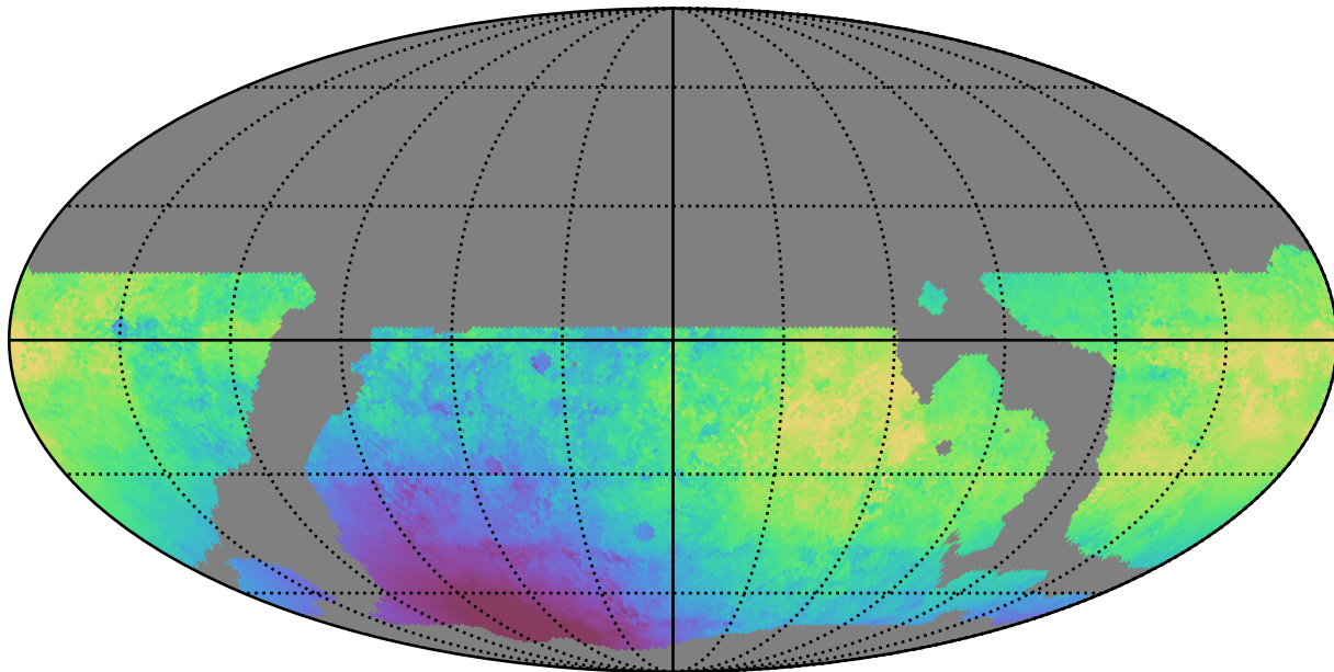
weather_cloudso18v3.4_10yrs WFD g band: Median solarElong
