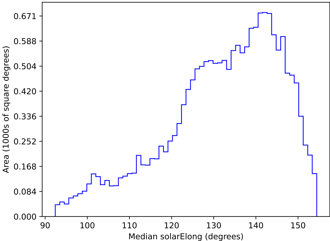
weather_cloudso18v3.4_10yrs WFD g band: Median solarElong
