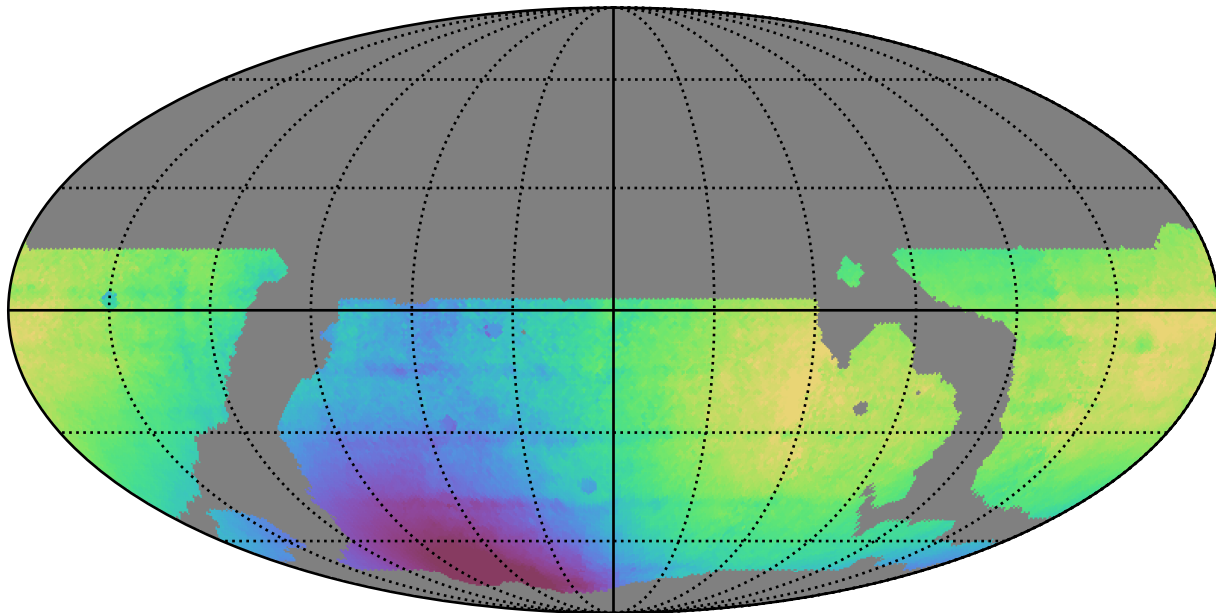
weather_cloudso18v3.4_10yrs WFD all bands: Median solarElong
