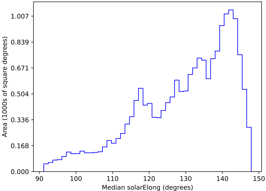
weather_cloudso18v3.4_10yrs WFD all bands: Median solarElong
