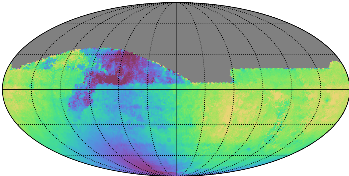
weather_cloudso18v3.4_10yrs All sky z band: Median solarElong
