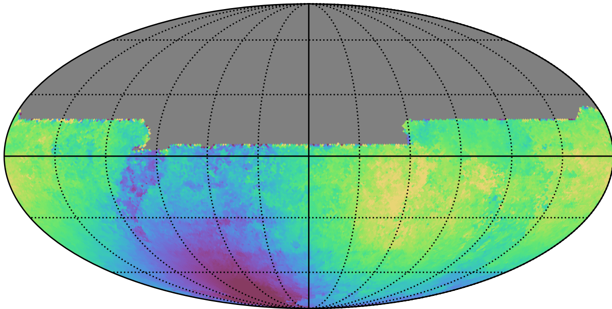
weather_cloudso18v3.4_10yrs All sky y band: Median solarElong
