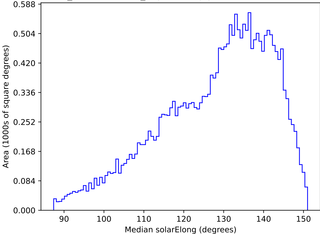
weather_cloudso18v3.4_10yrs All sky y band: Median solarElong
