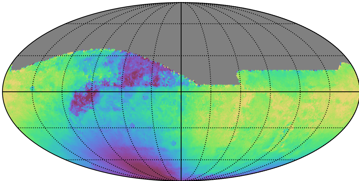
weather_cloudso18v3.4_10yrs All sky r band: Median solarElong
