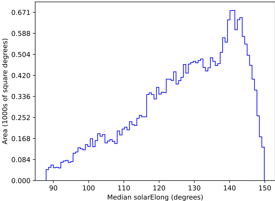
weather_cloudso18v3.4_10yrs All sky r band: Median solarElong
