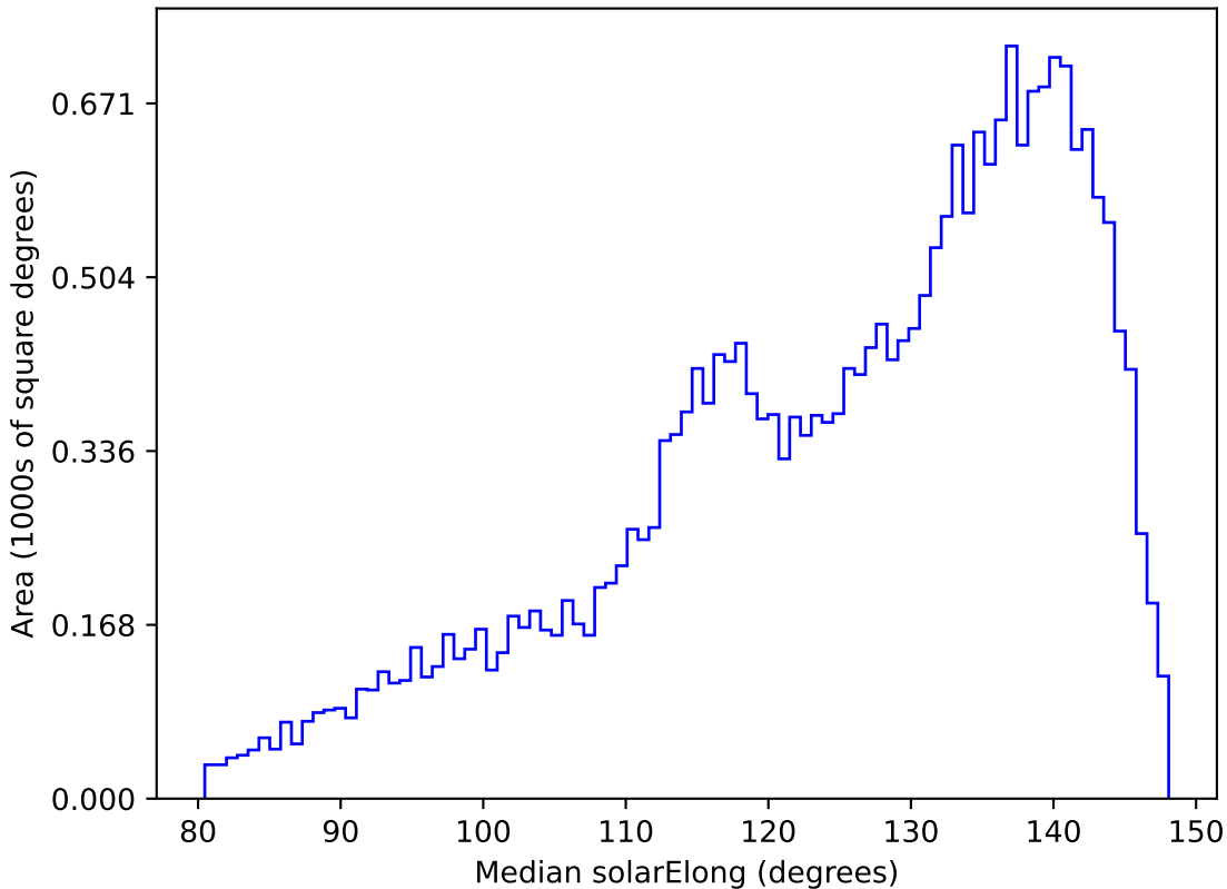
weather_cloudso18v3.4_10yrs All sky i band: Median solarElong
