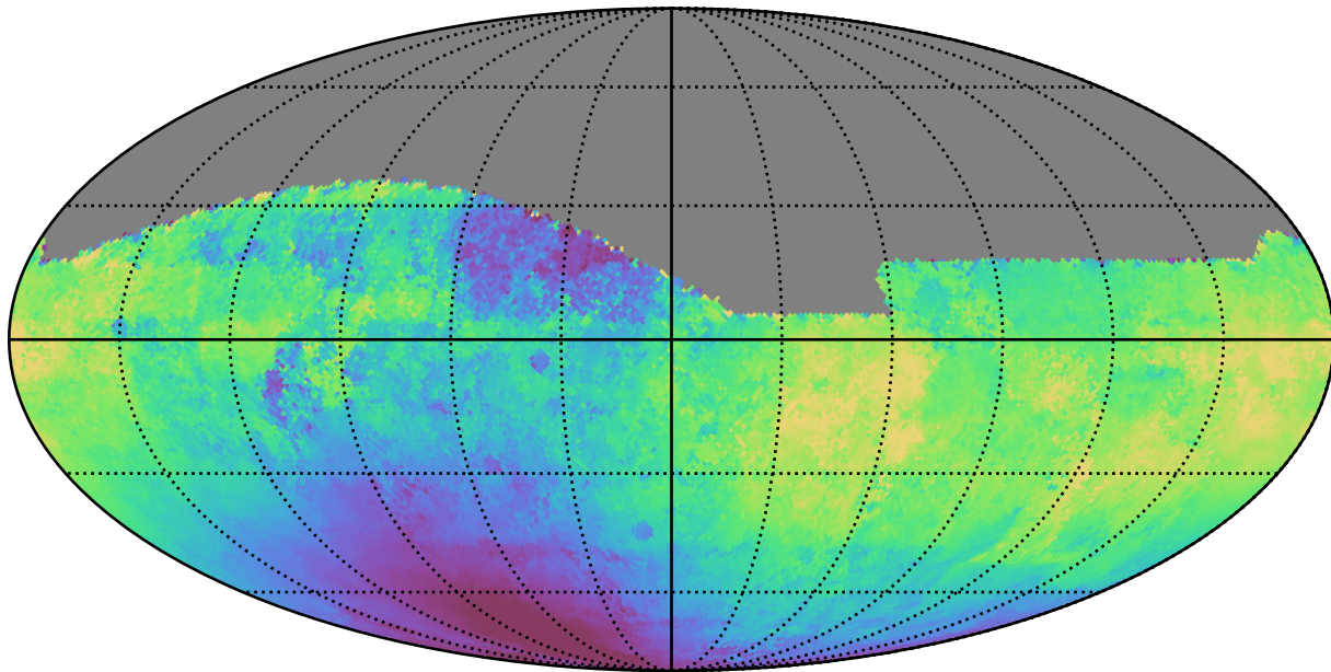
weather_cloudso18v3.4_10yrs All sky g band: Median solarElong
