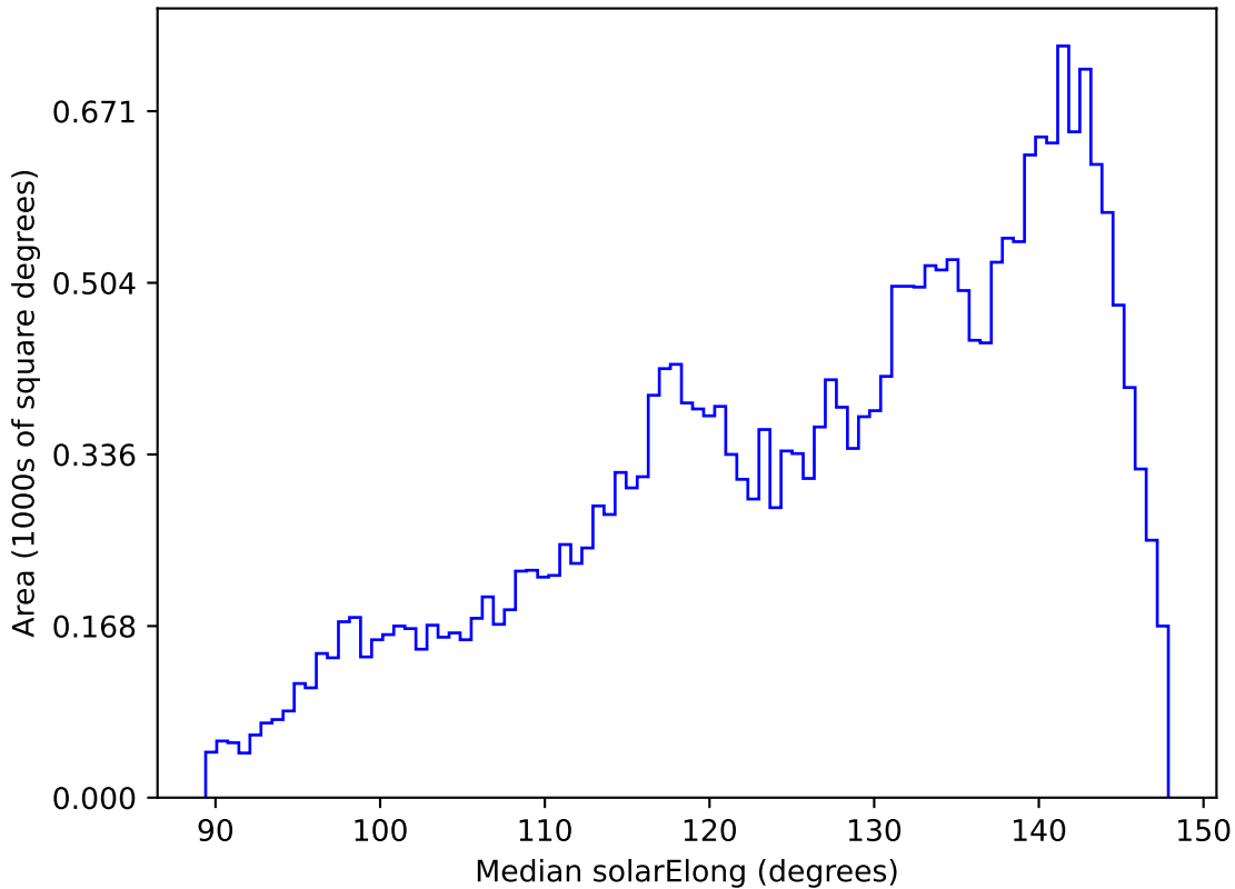
weather_cloudso18v3.4_10yrs All sky all bands: Median solarElong
