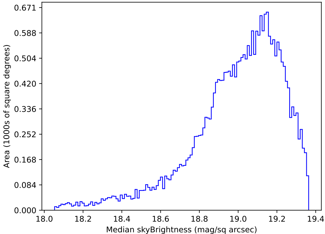
weather_cloudso18v3.4_10yrs Yr 1 z band: Median skyBrightness
