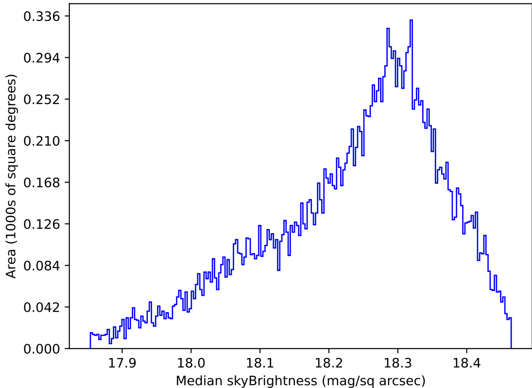
weather_cloudso18v3.4_10yrs Yr 1 y band: Median skyBrightness
