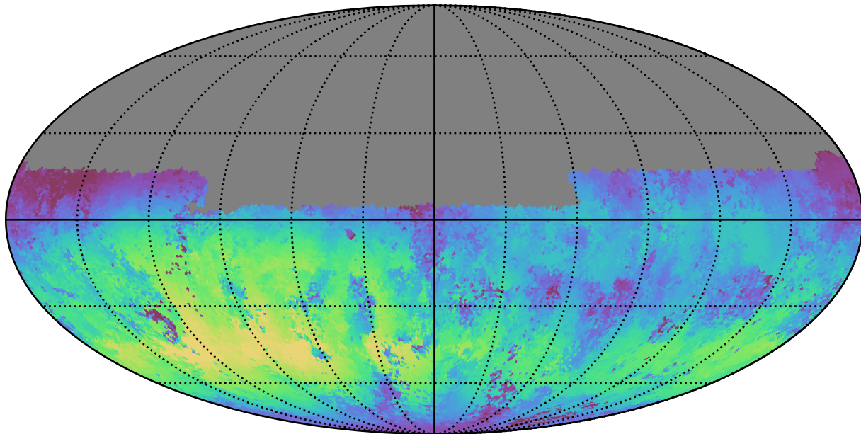
weather_cloudso18v3.4_10yrs Yr 1 u band: Median skyBrightness
