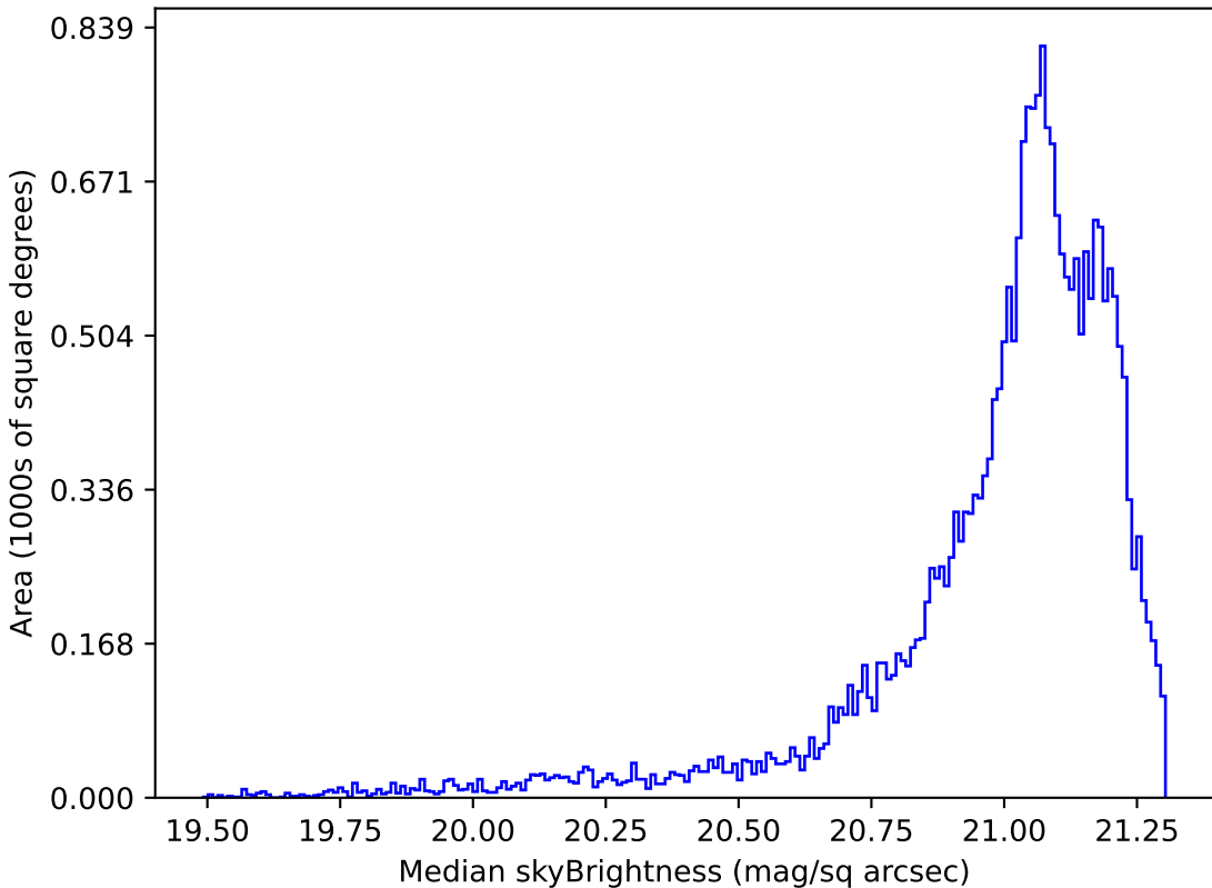
weather_cloudso18v3.4_10yrs Yr 1 r band: Median skyBrightness
