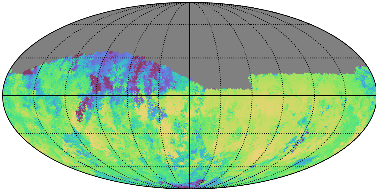
weather_cloudso18v3.4_10yrs Yr 1 i band: Median skyBrightness
