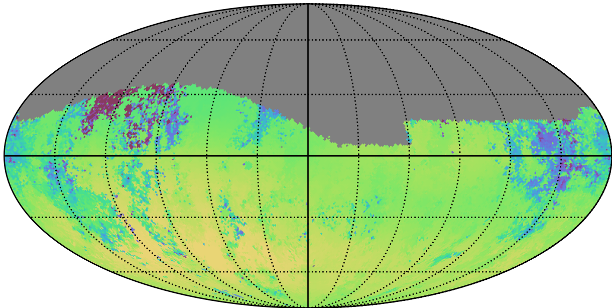
weather_cloudso18v3.4_10yrs Yr 1 g band: Median skyBrightness
