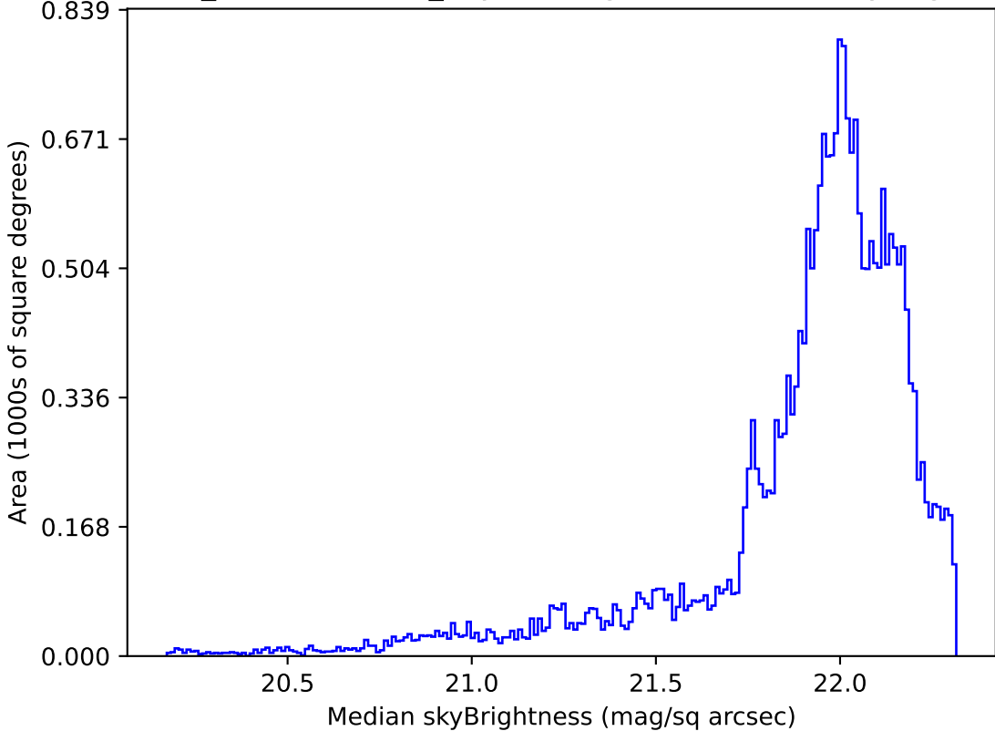
weather_cloudso18v3.4_10yrs Yr 1 g band: Median skyBrightness
