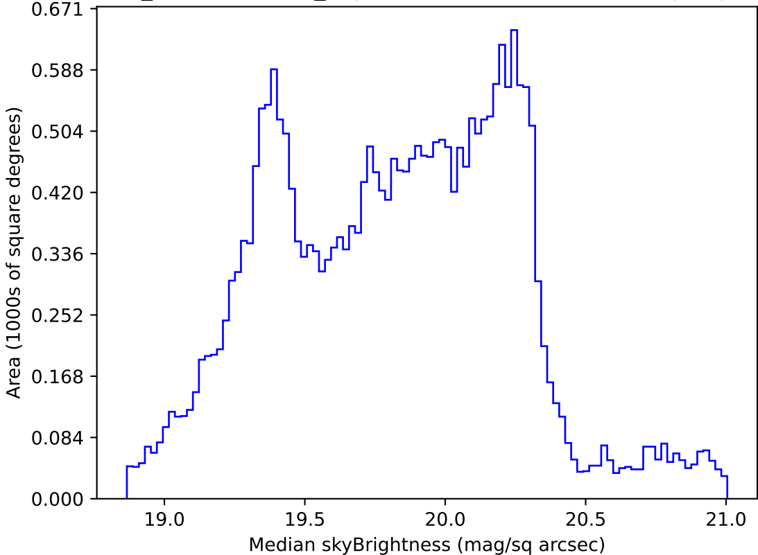
weather_cloudso18v3.4_10yrs Yr 1 all bands: Median skyBrightness
