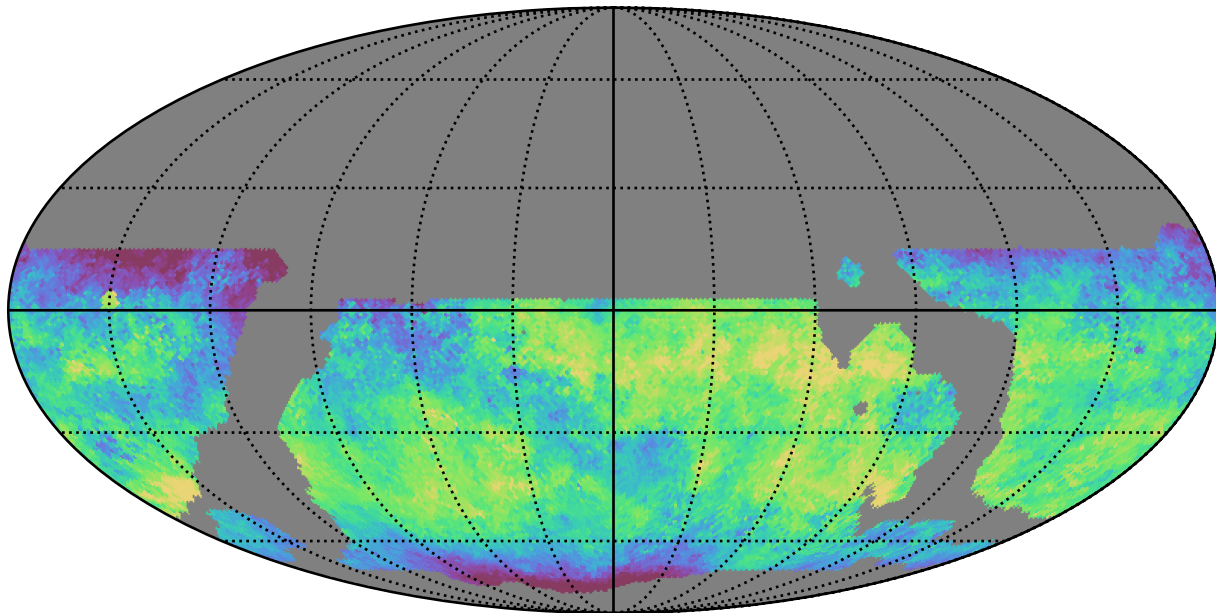
weather_cloudso18v3.4_10yrs WFD z band: Median skyBrightness
