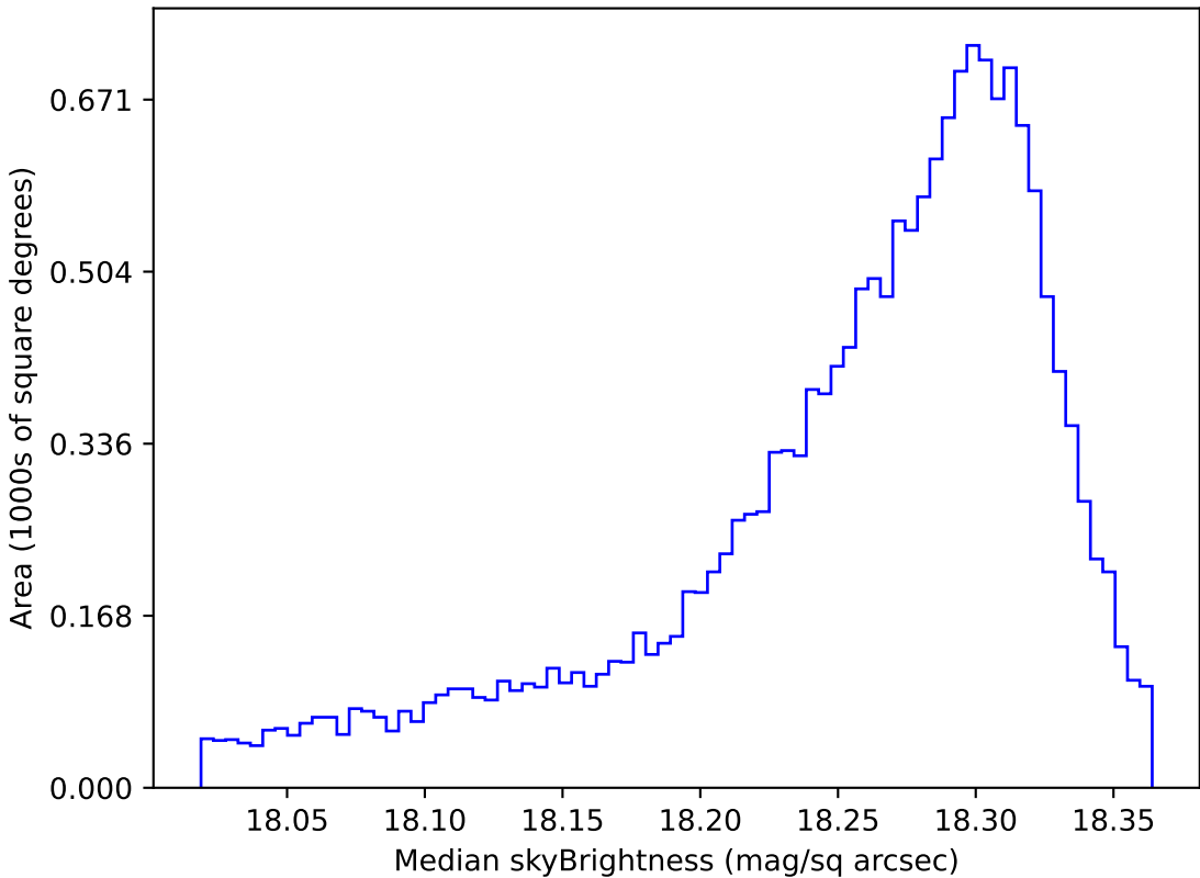
weather_cloudso18v3.4_10yrs WFD y band: Median skyBrightness
