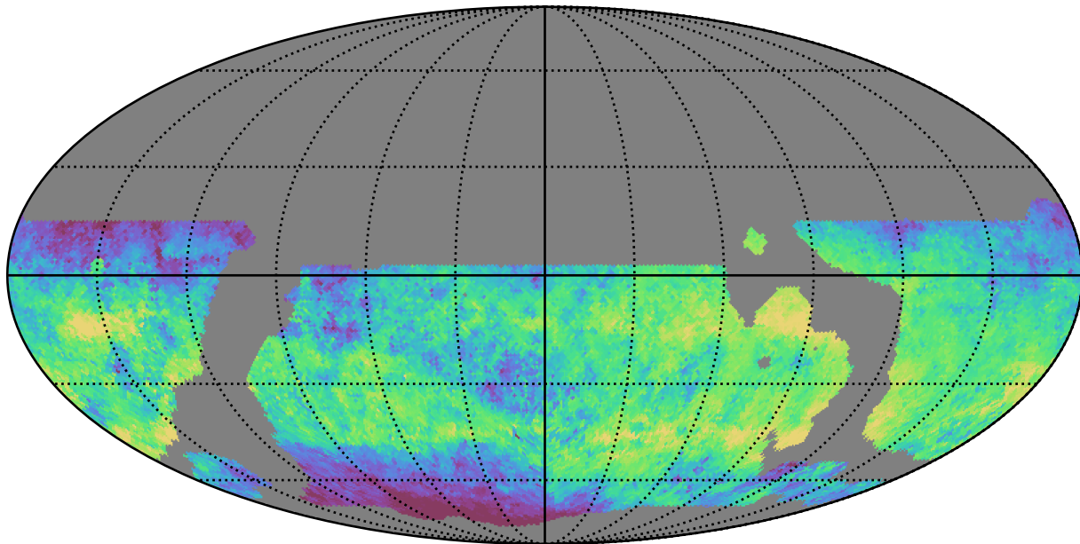
weather_cloudso18v3.4_10yrs WFD i band: Median skyBrightness
