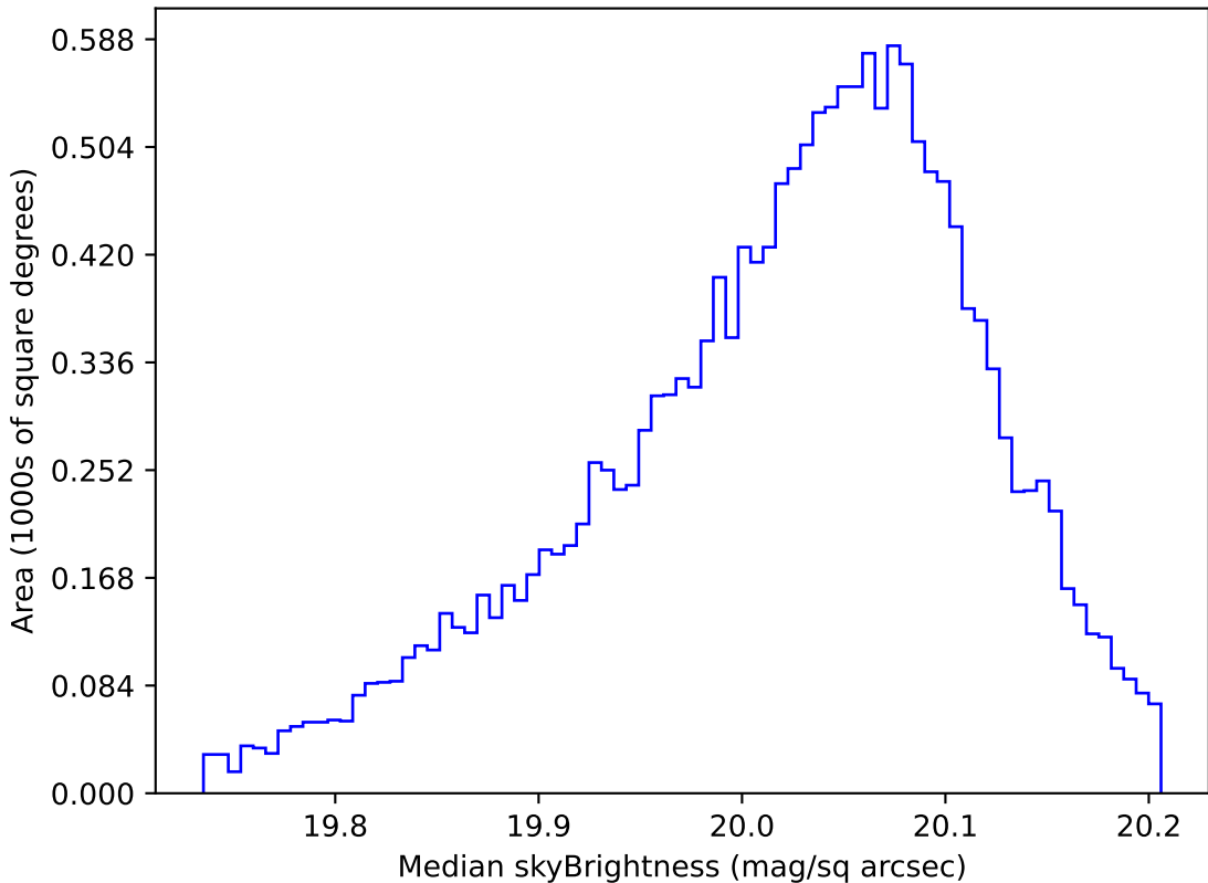
weather_cloudso18v3.4_10yrs WFD i band: Median skyBrightness
