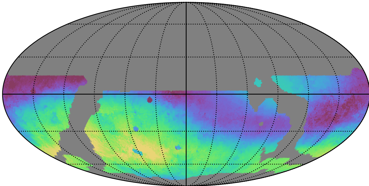
weather_cloudso18v3.4_10yrs WFD g band: Median skyBrightness
