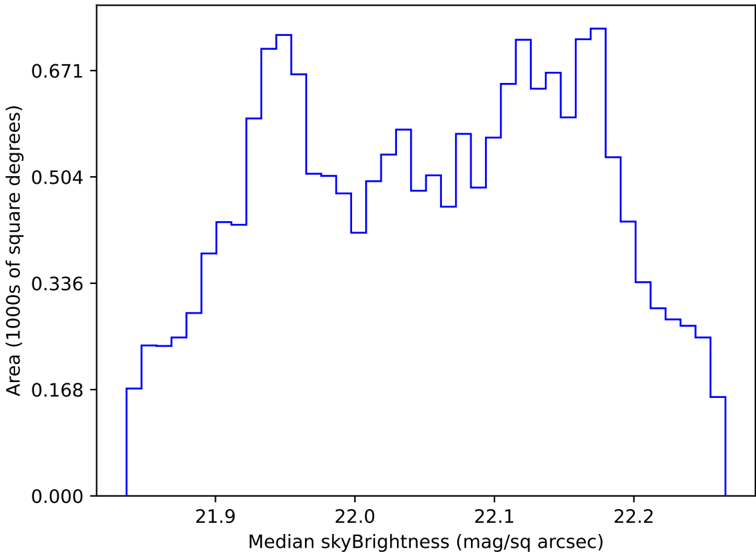
weather_cloudso18v3.4_10yrs WFD g band: Median skyBrightness
