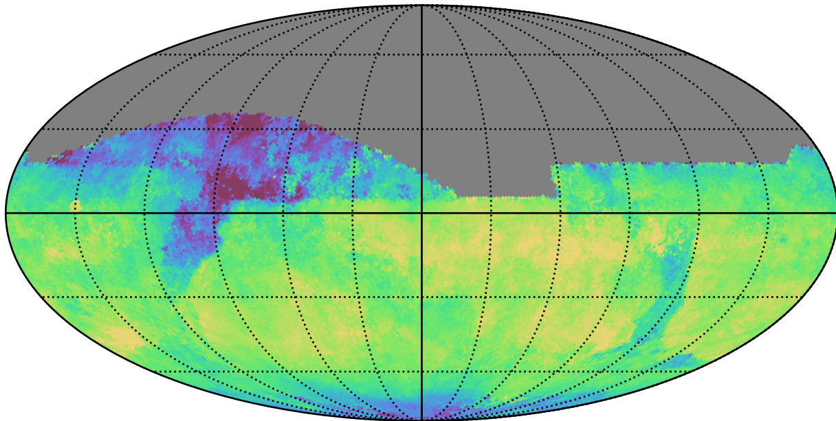
weather_cloudso18v3.4_10yrs All sky z band: Median skyBrightness
